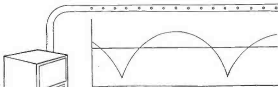
• Curve shows standing waves determined by probing electrostatic field in "piccolo" section of transmission line with holes drilled in outer conductor. Wavy curve represents initial conditions before adjustment; straight line shows the final result after adjustment of matching unit.
